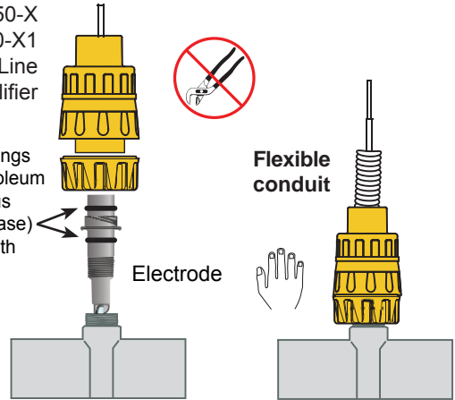
Signet Installation Fitting DN15 to DN100 (1/2 in. to 4 in.)
